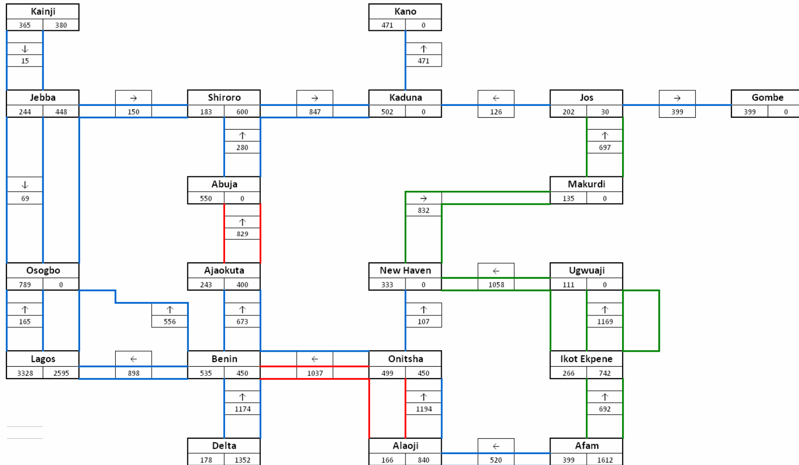
Figure 3: Projected load flow in excess of 8,500 MW (up to a maximum of circa 10,000 MW) with the completion of the Afam to Jos circuits plus the subsequent addition of the Onitsha to Benin circuits and the Alaoji-Warri-Onitsha circuits and the NIPP connection between Ajaokuta and Abuja
